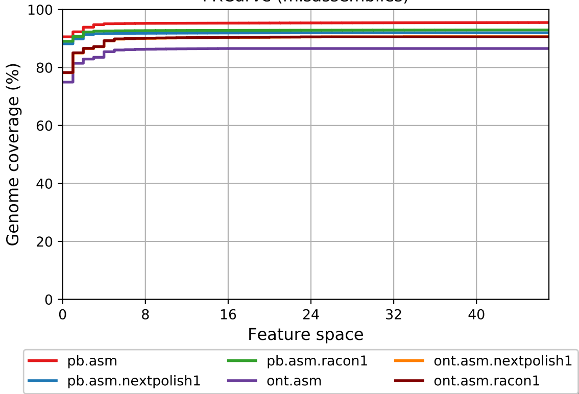
FRCurve (misassemblies)
