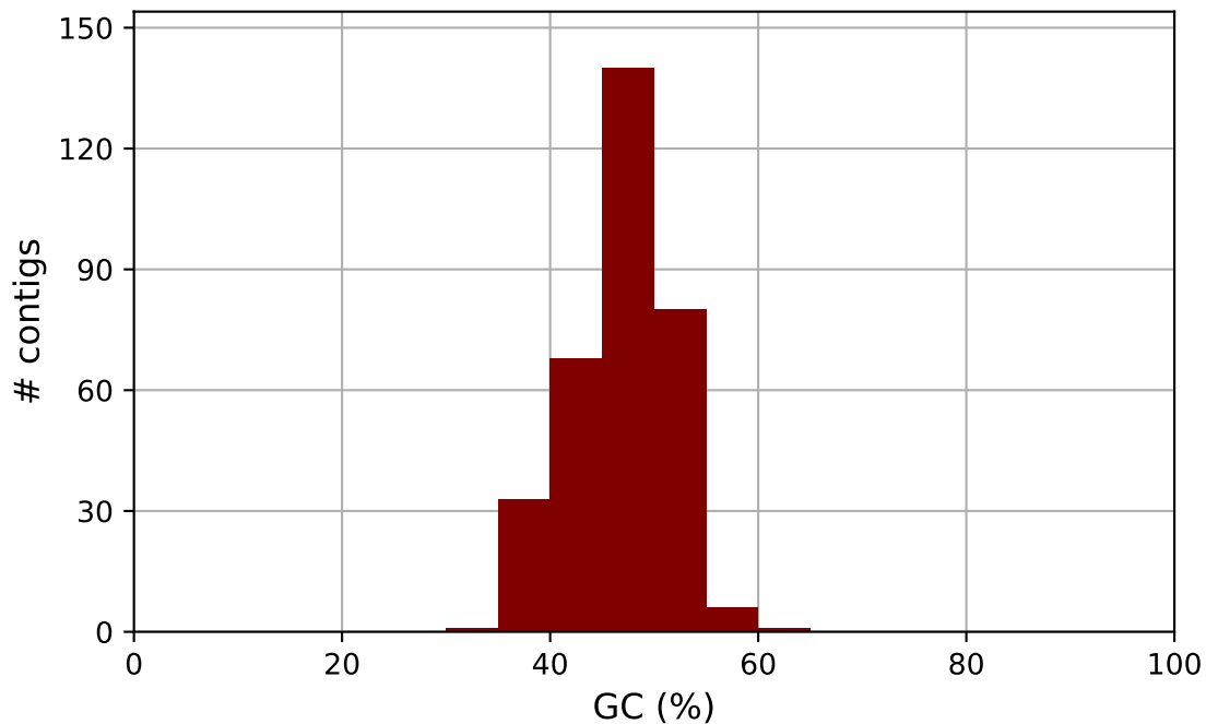
ont.asm.racon1 GC content
